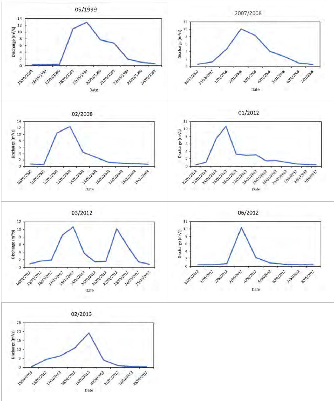
Figure 16-2: Hydrographs showing examples of flow events with peaks of ~10 m 3 /s that occurred in the Six Mile Creek Dam discharge record period 1999-2019
