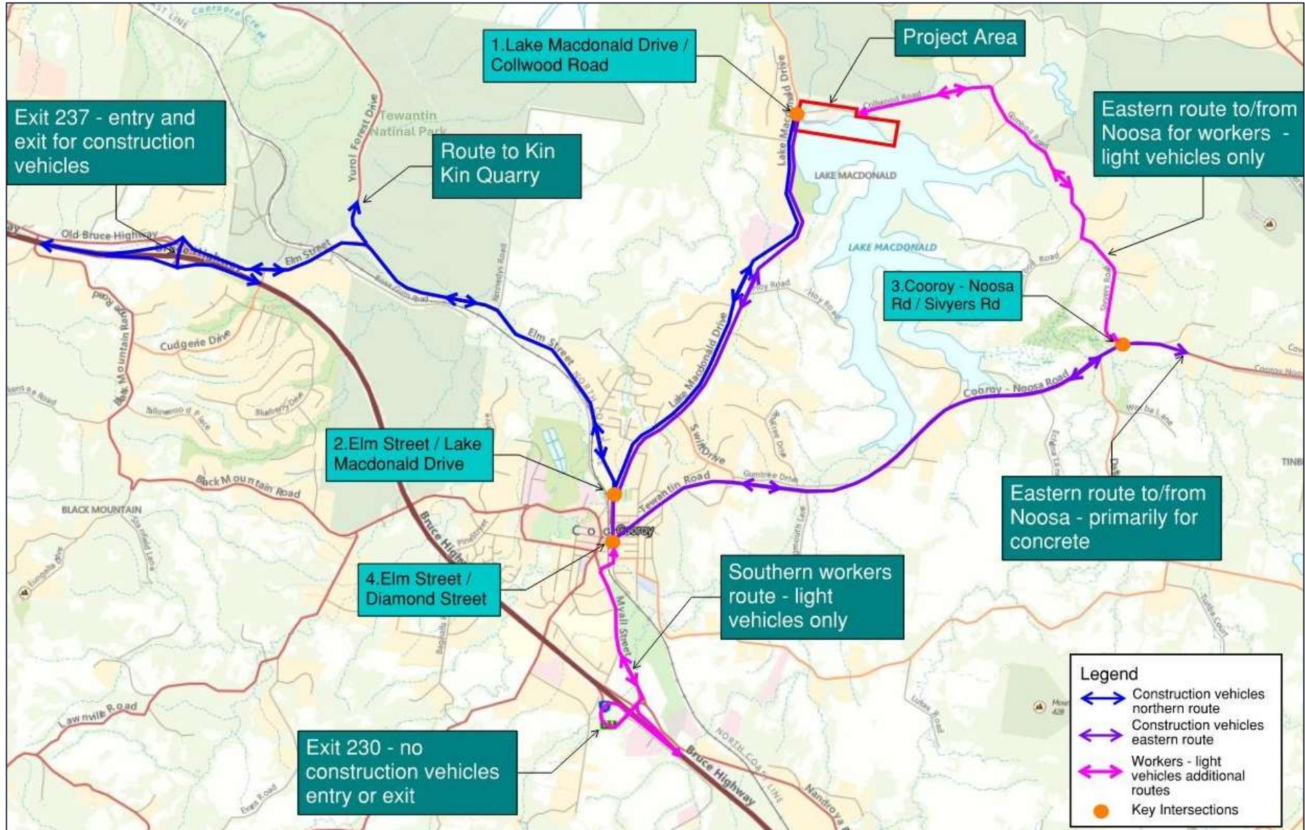
Figure 2-1: Site location, project vehicle routes and key intersections
